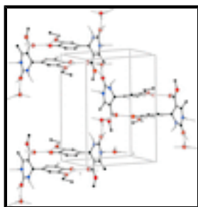
Fig. 2. Part of the crystal packing of the title compound, showing hydrogen-bonded (dashed lines) dimers.
